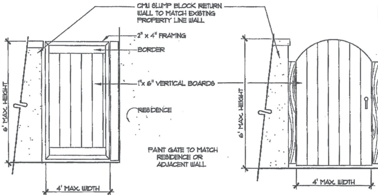
ARCHED WOOD GATE
